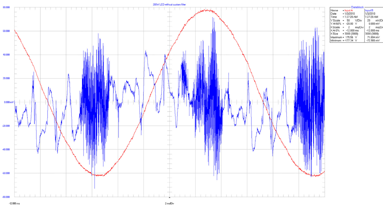
Fig. 6. The waveforms were collected at the Stetzer Electric offices in Blair, WI using a Fluke 190–202 Scopemeter. Channel A was connected to a 120 V receptacle. Channel B was connected at the same potential, except through the Graham Ubiquitous Filter (removes the 60 cycle). A 200 W LED light fixture without custom filter was in use at the time.
