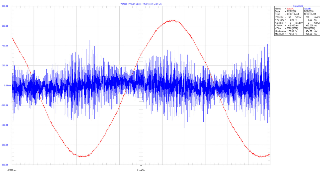
Fig. 4. The waveforms were collected at the Stetzer Electric offices in Blair, WI using a Fluke 190–202 Scopemeter. Channel A was connected to a 120 V receptacle. A collapsible antenna on B Channel was measuring voltage through the air. The 4-foot, 6-lamp T8 fluorescent light was on at the time. Measurements were taken with the scope placed approximately 6 feet from the fluorescent light.
