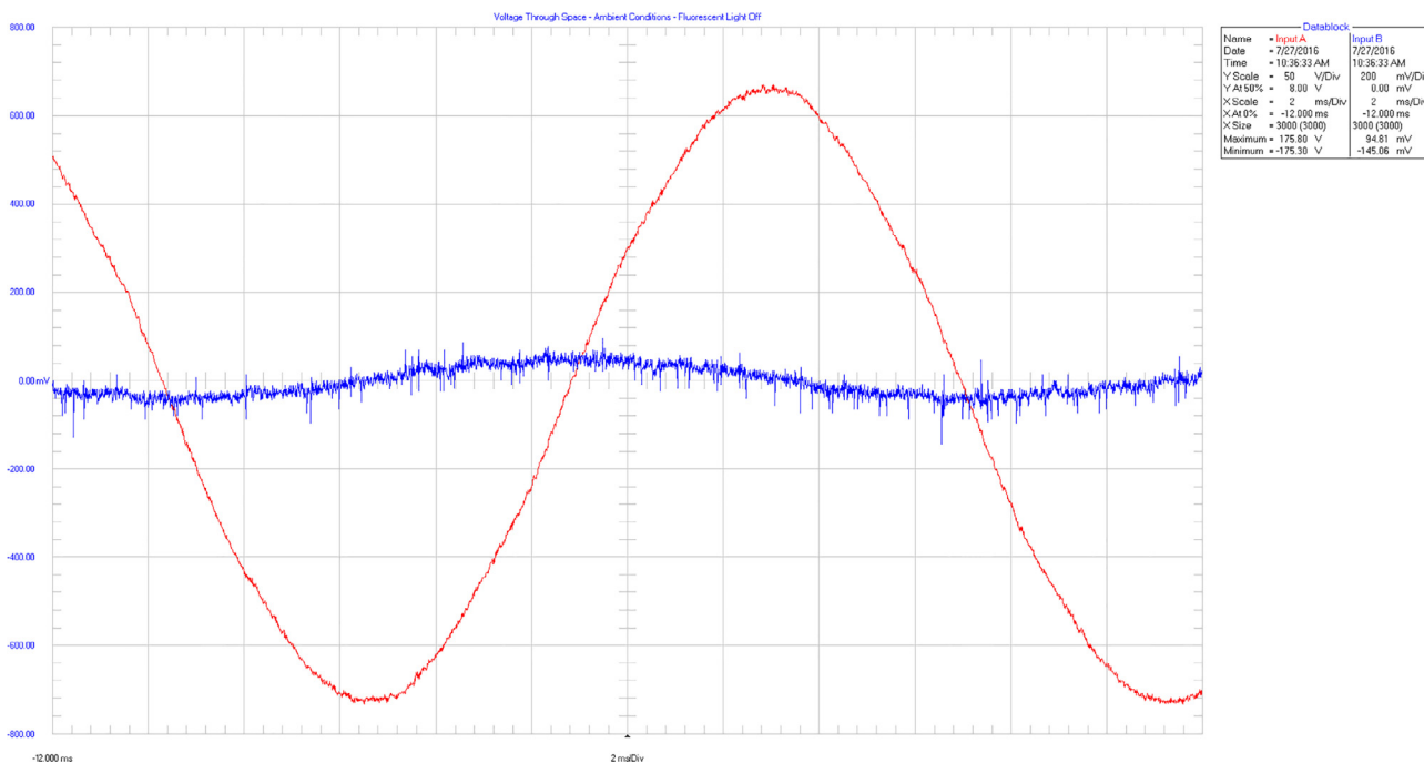
Fig. 5. The waveforms were collected at the Stetzer Electric offices in Blair, WI using a Fluke 190–202 Scopemeter. Channel A was connected to a 120 V receptacle. A collapsible antenna on B Channel was measuring voltage through the air. The 4-foot, 6-lamp T8 fluorescent light was off at the time. Measurements were taken with the scope placed in the same location as when the fluorescent light was turned on.
